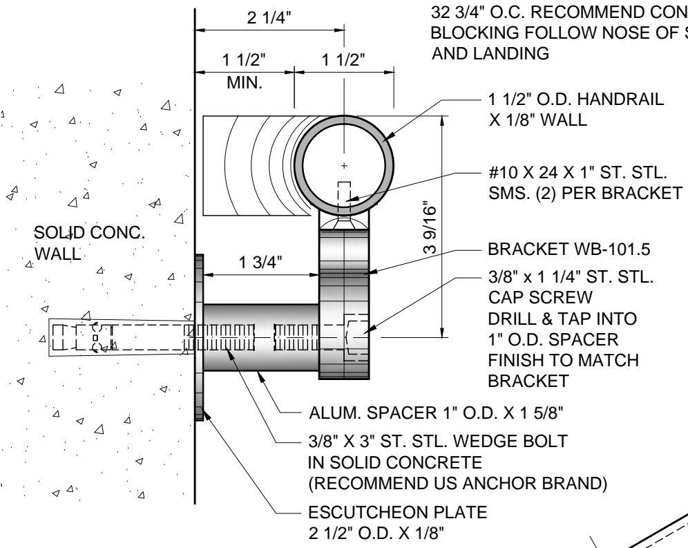
C BRACKET SECTION SCALE: HALF SIZE
