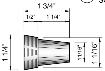
ALTERNATE SPACER PART NO. S-101C
